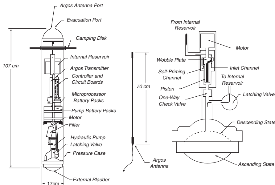
Figure 10.14 The Autonomous Lagrangean Circulation Explorer (ALACE) drifters are widely used by the World Ocean Circulation Experiment to measure deeper currents within the ocean. Left: Schematic of the drifter. To ascend, the hydraulic pump moves oil from an internal reservoir to an external bladder, reducing the drifter's density. To descend, the latching valve is opened to allow oil to flow back into the internal reservoir. The antenna is mounted to the end cap. Right: Expanded schematic of the hydraulic system. The motor rotates the wobble plate actuating the piston which pumps hydraulic oil. (From Davis et al., 1992).
