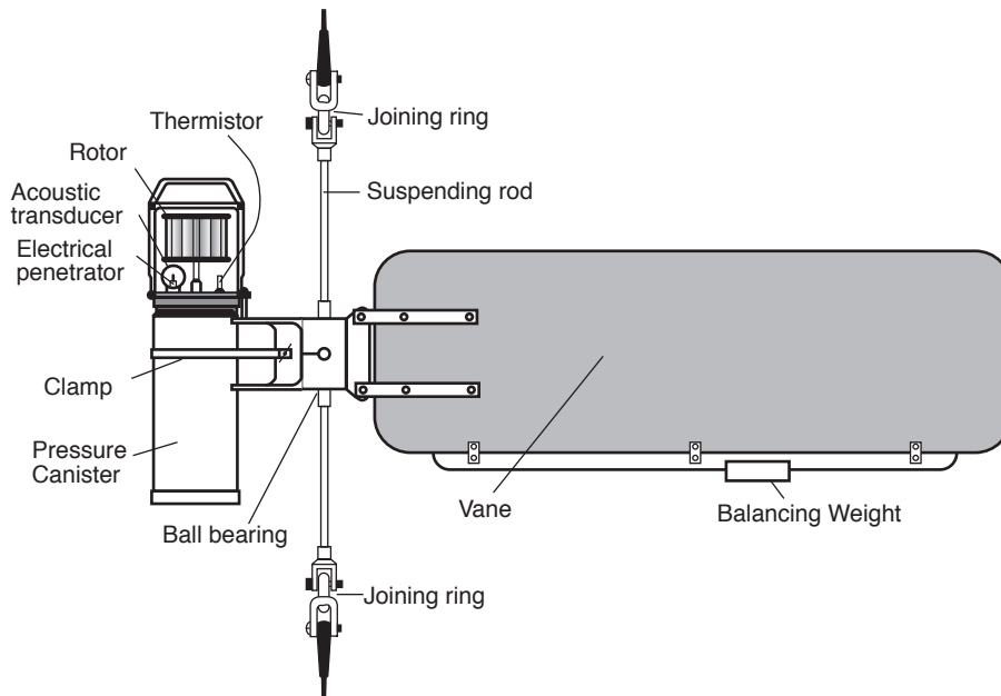
Figure 10.19 An example of a moored current meter with a Savonius rotor to measure current speed, a vane to measure current direction, and a pressure-resistant housing for power and circuits to record the signal. The turns of the rotor are measured by the acoustic transducer. (From Dietrich, et al. 1980)
