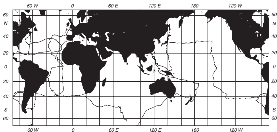
Figure 2.1 Example from the era of deep-sea exploration: Track of H.M.S. Challenger during the British Challenger Expedition 1872–1876 (From Wust, 1964).
