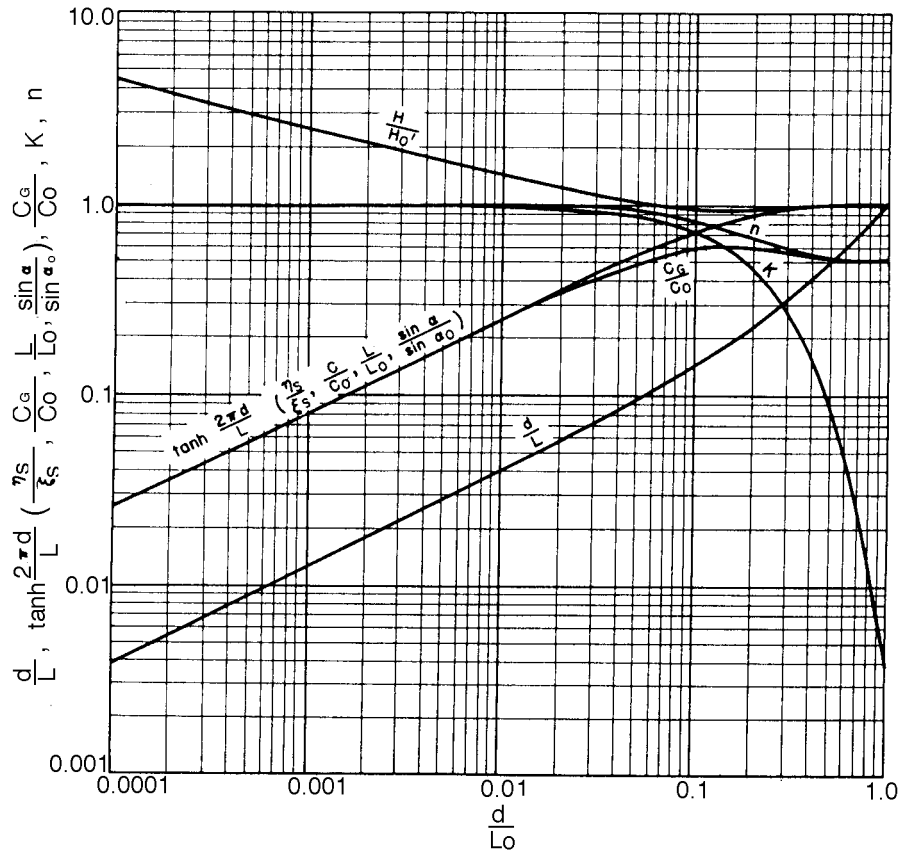
Figure 17.1 Change in wave properties as waves shoal (From Wiegel, 1964).
