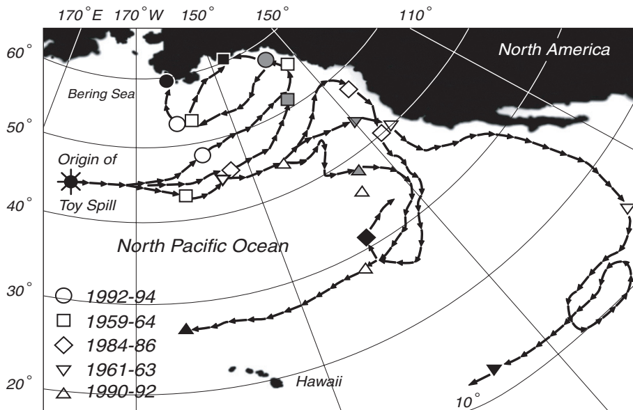
Figure 10.17 Trajectories that spilled rubber duckies would have followed had they been spilled on January 10 of different years. Five trajectories were selected from a set of 48 simulations of the spill each year between 1946 and 1993. The trajectories begin on January 10 and end two years later (solid symbols). Grey symbols indicate positions on November 16 of the year of the spill. Hence the grey circle gives the location where rubber ducks first came ashore near Sitka. The code at lower left gives the dates of the trajectories. (From Ebbesmeyer and Ingraham, 1994).
