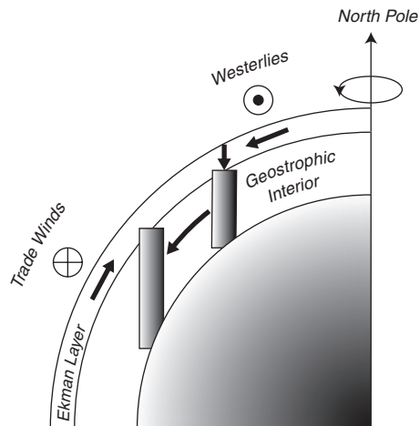
Figure 12.6 Ekman pumping that produces a downward velocity at the base of the Ekman layer forces the fluid in the interior of the ocean to move southward. (From Niiler, 1987)
