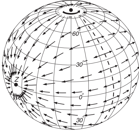
Figure 17.11 The horizontal component of the tidal force on earth when the tide-generating body is above the Equator at Z . (From Dietrich, et.al., 1980).
