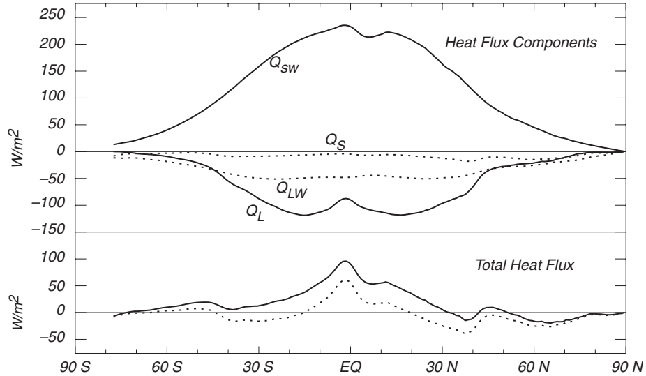
Figure 5.7 Upper: Zonal averages of heat transfer to the ocean by insolation Q_{SW} , and loss by infrared radiation Q_{LW} , sensible heat flux Q_S , and latent heat flux Q_L , calculated by DaSilva, Young, and Levitus (1995) using the COADS data set. Lower: Net heat flux through the sea surface calculated from the data above (solid line) and net heat flux constrained to give heat and fresh-water transports by the ocean that match independent calculations of these transports. The area under the lower curves ought to be zero, but it is 16 \text{ W/m}^2 for the unconstrained case and -3 \text{ W/m}^2 for the constrained case.
