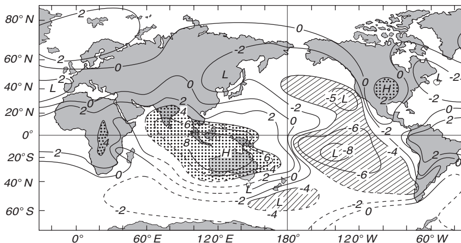
Figure 14.6 Correlation coefficient of annual-mean sea-level pressure with pressure at Darwin. - - - - Coefficient < -0.4 . (From Trenberth and Shea, 1987).
