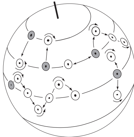
Figure 12.3 Angular momentum tends to be conserved as columns of water change latitude. This causes changes in relative vorticity of the columns (from von Arx, 1962).
