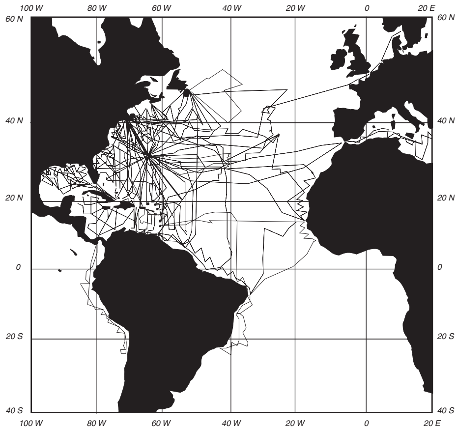
Figure 2.3 Example from the era of new methods. The cruises of the R/V Atlantis out of Woods Hole Oceanographic Institution (From Wust, 1964).
