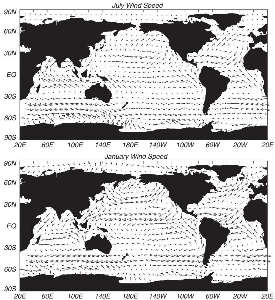
Figure 4.4 Mean, sea-surface winds for July and January calculated by Trenberth's (1990) data set calculated from the ECMWF reanalyses of weather data from 1980 to 1989.
