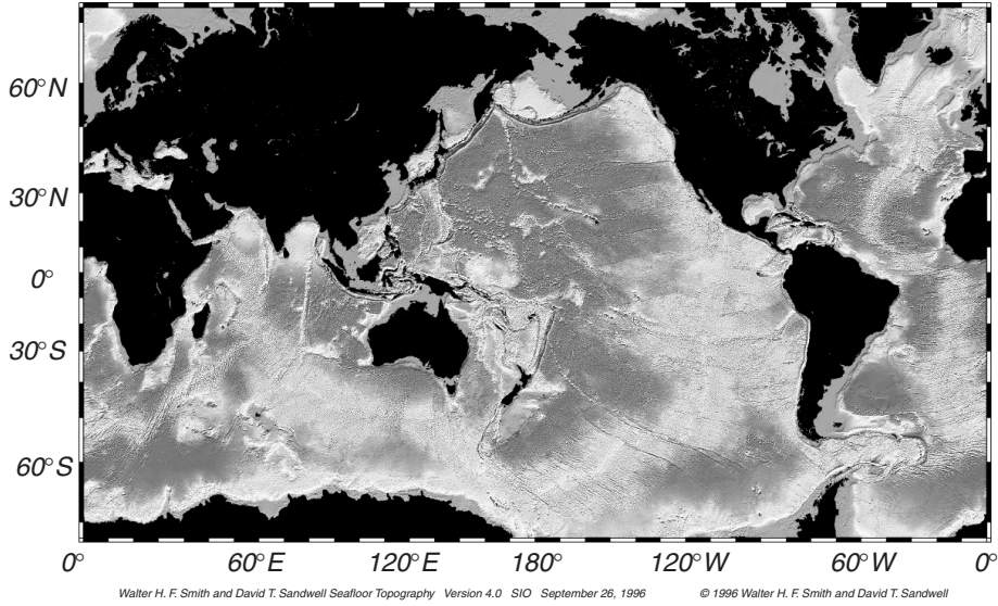
Figure 3.14 The sea-floor topography of the ocean with 3 km resolution produced from satellite altimeter observations of the shape of the sea surface (From Smith and Sandwell).
