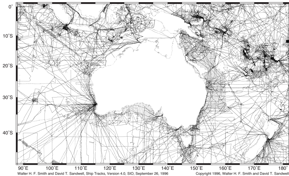
Figure 3.11 Locations of echo-sounder data used for mapping the ocean floor near Australia. Note the large areas where depths have not been measured from ships. (From Sandwell)
