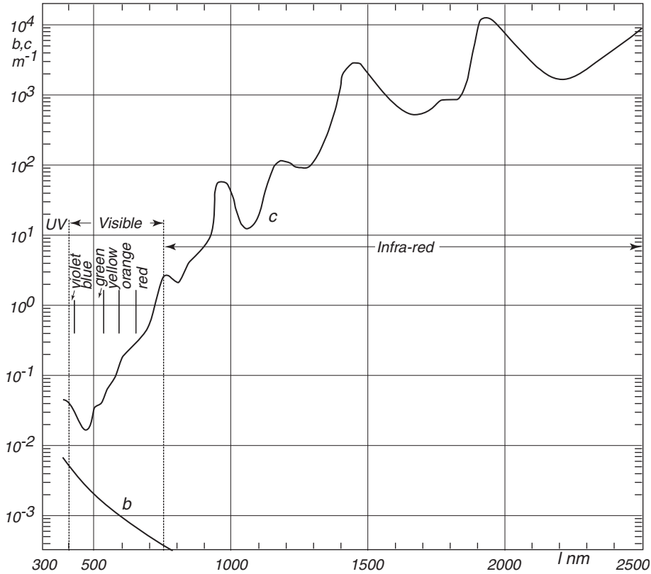
Figure 6.17 Attenuation coefficient c and scattering coefficient b for pure water as a function of wavelength \lambda of the radiation (From Dietrich, et al. 1980).
