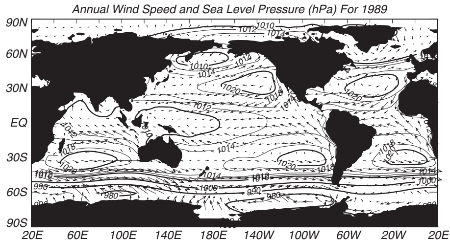
Figure 4.2 Map of mean annual wind velocity calculated from Trenberth (1990) and sea-level pressure for 1989 from the NASA Goddard Space Flight Center's Data Assimilation Office (Schubert et al. 1995).
