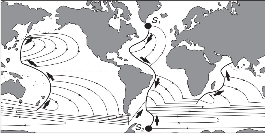
Figure 13.4 Sketch of the deep circulation resulting from deep convection in the Atlantic (dark circles) and upwelling through the thermocline elsewhere (After Stommel, 1958).
