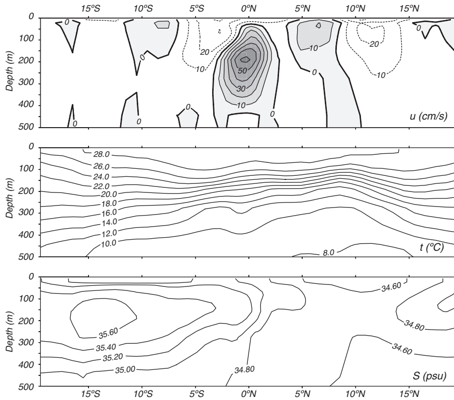
Figure 14.4 Cross section of the Equatorial Undercurrent in the Pacific calculated from Modular Ocean Model with assimilated surface data (See §14.5). The section an average from 160°E to 170°E from January 1965 to December 1999. Stippled areas are westward flowing. (From Nevin Fuckar).
