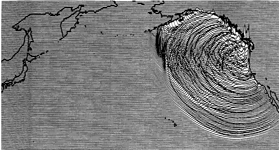
Figure 17.8 Tsunami wave height four hours after the great M9 Cascadia earthquake off the coast of Washington on 26 January 1700 calculated by a finite-element, numerical model. Maximum open-ocean wave height, about one meter, is north of Hawaii (From Satake et al 1996).
