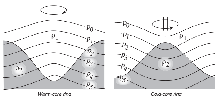
Figure 10.12 Shape of constant-pressure surfaces p_i and the interface between two water masses of density \rho_1, \rho_2 if the upper is rotating faster than the lower. Left: Anticyclonic motion, warm-core eddy. Right: Cyclonic, cold-core eddy. Note that the sea surface p_0 slopes up toward the center of the warm-core ring, and the constant-density surfaces slope down toward the center (From Defant, 1929).
