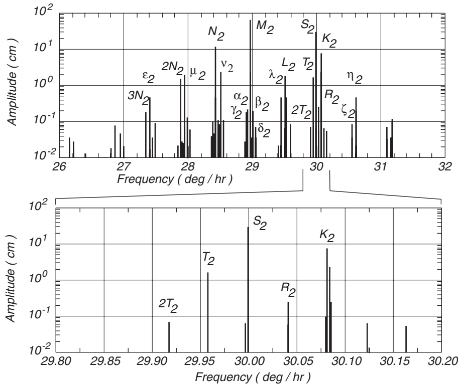
Figure 17.12 Upper: Spectrum of equilibrium tides with frequencies near twice per day. The spectrum is split into groups separated by a cycle per month (0.55 deg/hr). (Lower: Expanded spectrum of the S_2 group, showing splitting at a cycle per year (0.04 deg/hr). The finest splitting in this figure is at a cycle per 8.847 years (0.0046 deg/hr).
