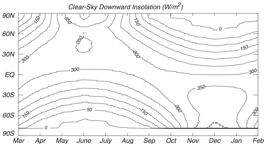
Figure 5.3 Monthly average of downward flux of sunlight through a cloud-free sky and into the ocean in W/m^2 during 1989 calculated by the Satellite Data Analysis Center at the NASA Langley Research Center (Darnell et al. 1992) using data from the International Satellite Cloud Climatology Project.
