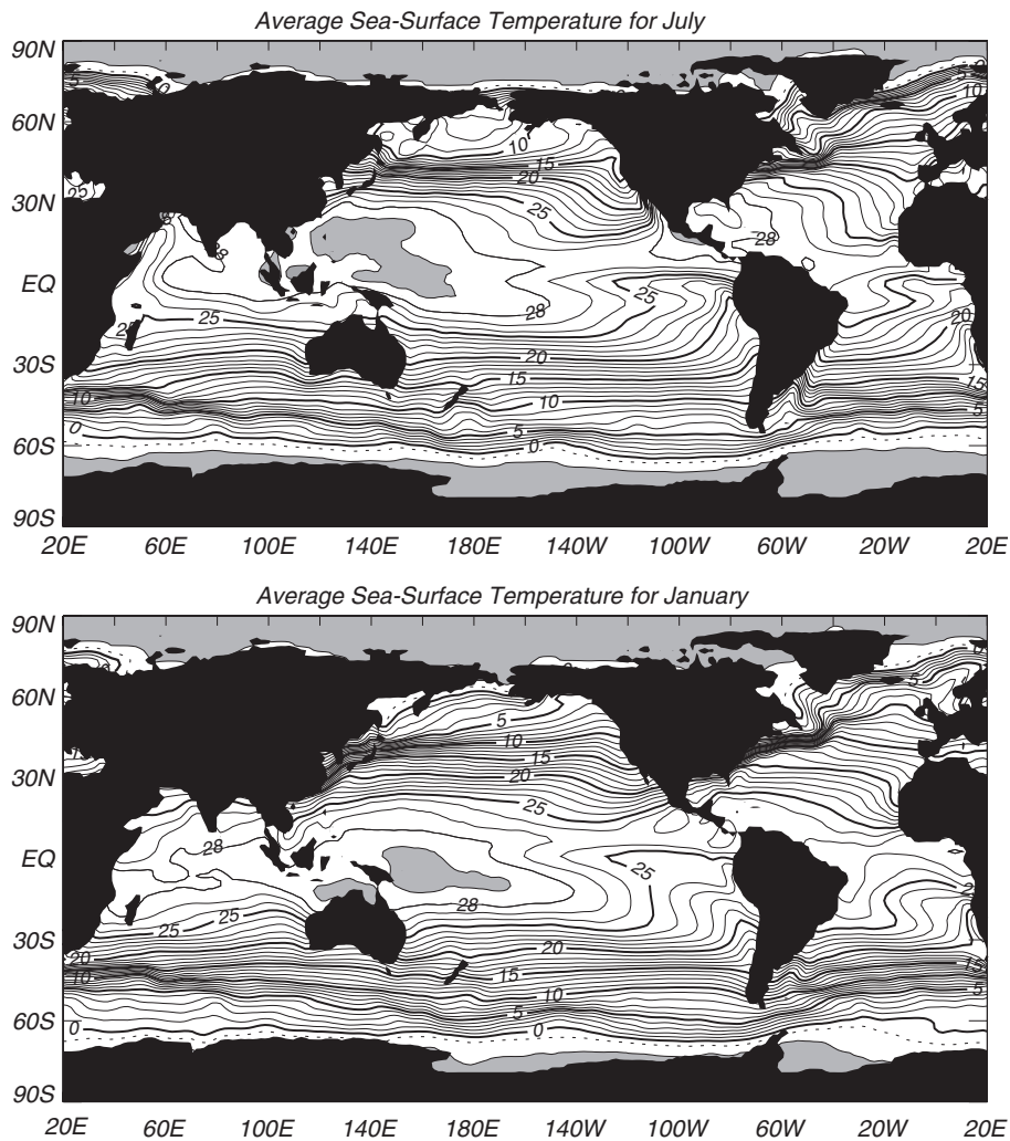
Figure 6.2 Mean sea-surface temperature calculated from the optimal interpolation technique (Reynolds and Smith, 1995) using ship reports and AVHRR measurements of temperature. Contour interval is 1^{\circ}\text{C} with heavy contours every 5^{\circ}\text{C} . Shaded areas exceed 29^{\circ}\text{C} .
