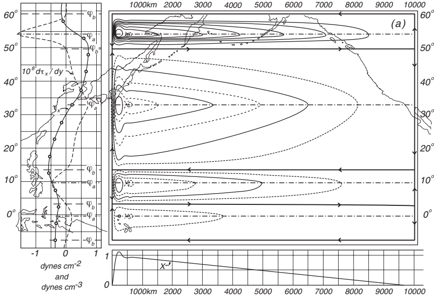
Figure 11.6 Upper Left: Mean annual wind stress T_x(y) over the Pacific and the curl of the wind stress. \varphi_b are the northern and southern boundaries of the gyres, where M_y = 0 and curl \tau = 0 . \varphi_0 is the center of the gyre. Upper Right: The mass transport stream function for a rectangular basin calculated by Munk (1950) using observed wind stress for the Pacific. Contour interval is 10 Sverdrups. The total transport between the coast and any point x, y is \psi(x, y) . The transport in the relatively narrow northern section is greatly exaggerated. Lower Right: North-South component of the mass transport (From Munk, 1950).
