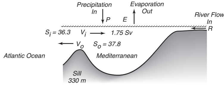
Figure 7.1 Schematic diagram of flow into and out of a basin. From Pickard and Emery, 1990.
