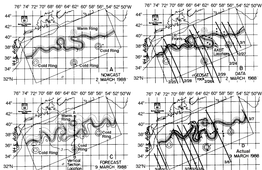
Figure 15.5 Output from the Harvard Open-Ocean Model: A the initial state of the model, the analysis, and B Data used to produce the analysis for 2 March 1988. C The forecast for 9 March 1988. D The analysis for 9 March. Although the Gulf Stream changed substantially in one week, the model forecasts the changes well. (From Robinson et al. 1989)
