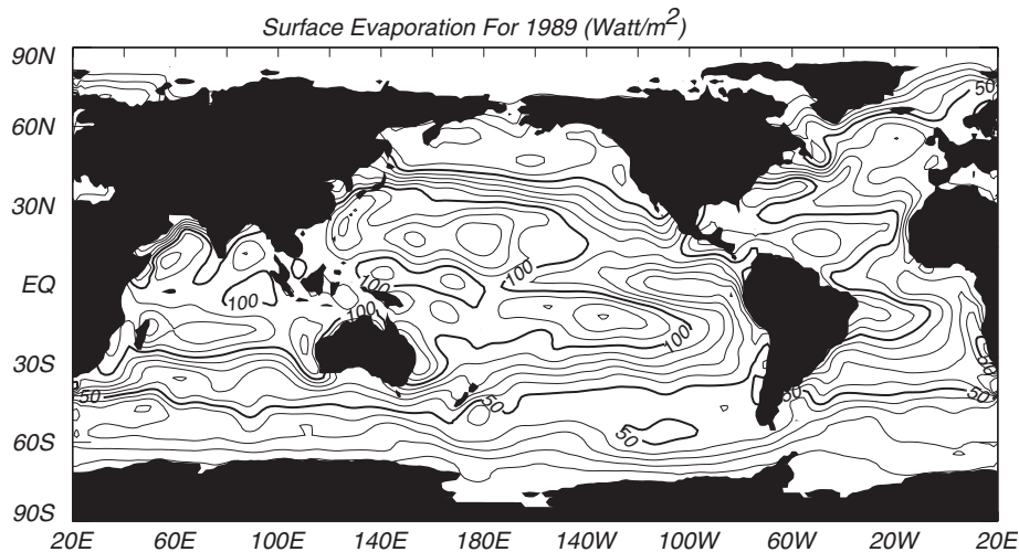
Figure 5.9 Annual-mean latent heat flux from the sea surface Q_L in W/m^2 during 1989 calculated from data compiled by the Data Assimilation Office of NASA's Goddard Space Flight Center using reanalyzed output from the ECMWF numerical weather prediction model. Contour interval is 10 W/m^2 .
