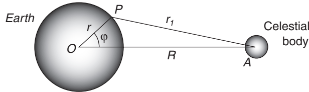
Figure 17.10 Sketch of coordinates for determining the tide-generating potential.
