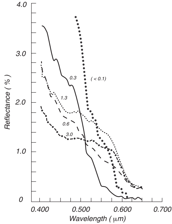
Figure 6.19 Spectral reflectance of sea water observed from an aircraft flying at 305 m over waters of different colors in the Northwest Atlantic. The numerical values are the average chlorophyll concentration in the euphotic (sunlit) zone in units of \text{mg}/\text{m}^3 . The reflectance is for vertically polarized light observed at Brewster's angle of 53^\circ . This angle minimizes reflected skylight and emphasizes the light from below the sea surface (From Clarke, Ewing, and Lorenzen, 1970).
