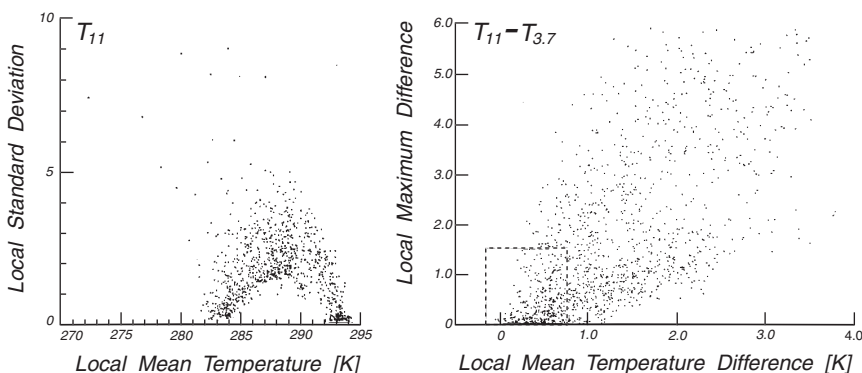
Figure 6.12 The influence of clouds on infrared observations. Left: The standard deviation of the radiance from small, partly cloudy areas each containing 64 pixels. The feet of the arch-like distribution of points are the sea-surface and cloud-top temperatures. (After Coakley and Bretherton (1982). Right: The maximum difference between local values of T_{11} - T_{3.7} and the local mean values of the same quantity. Values inside the dashed box indicate cloud-free pixels. T_{11} and T_{3.7} are the apparent temperatures at 11.0 and 3.7 \mu\text{m} (data from K. Kelly). From Stewart (1985).
