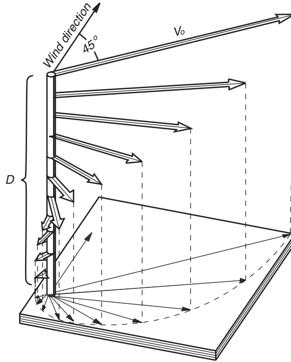
Figure 9.3. Vertical distribution of current due to wind blowing on the sea surface (From Dietrich, et al. , 1980).
