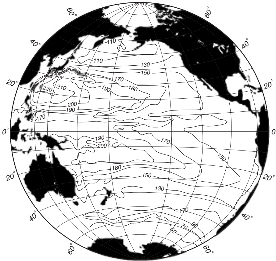
Figure 10.9. Mean depthgeopotential anomaly of the Pacific Ocean relative to the 1,000 dbar surface based on 36,356 observations. Height is in geopotential centimeters. If the velocity at 1,000 dbar were zero, the map would be the surface topography of the Pacific. (From Wyrski, 1974).
