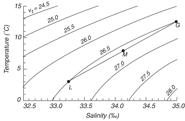
Figure 13.8 Mixing of two water types of the same density(L and G) produces water that is denser (M) than either water type. From Tolmazin (1985).
