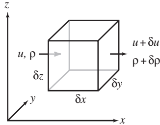
Figure 7.5 Sketch of flow used for deriving the continuity equation.
