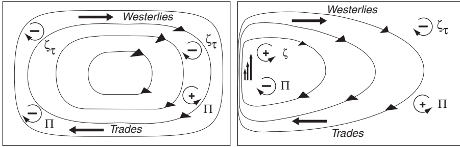
Figure 12.5 The balance of potential vorticity can clarify why western boundary currents are necessary. Left: Vorticity input by the wind \zeta_\tau balances the change in potential vorticity \Pi in the east as the flow moves southward and f decreases. The two do not balance in the west where \Pi must decrease as the flow moves northward and f increases. Right: Vorticity in the west is balanced by relative vorticity \zeta generated by shear in the western boundary current.
