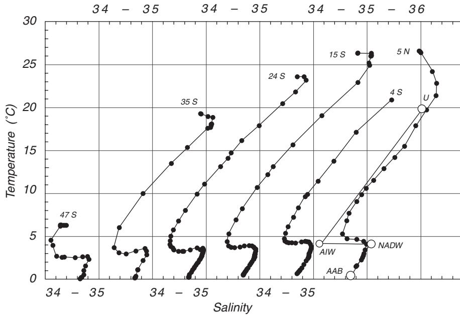
Figure 13.9 T-S plot of data collected at various latitudes in the western basins of the south Atlantic. Lines drawn through data from 5°N, showing possible mixing between water masses: NADW–North Atlantic Deep Water, AIW–Antarctic Intermediate Water, AAB Antarctic Bottom Water, U Subtropical Lower Water.
