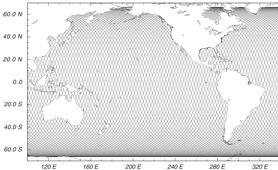
Figure 2.6 Example from the era of satellites. Topex/Poseidon tracks in the Pacific Ocean during a 10-day repeat of the orbit.
