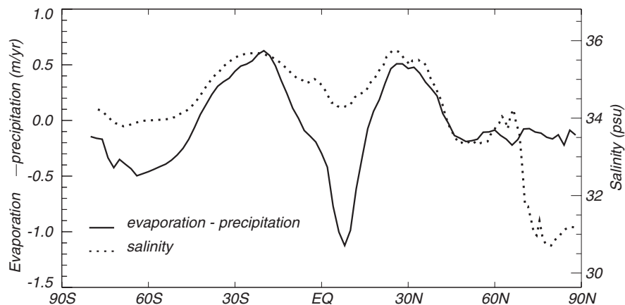
Figure 6.5 Zonal average of sea-surface salinity calculated for all oceans from Levitus (1982) and the difference between evaporation and precipitation ( E - P ) calculated from data shown in figure 5.14.
