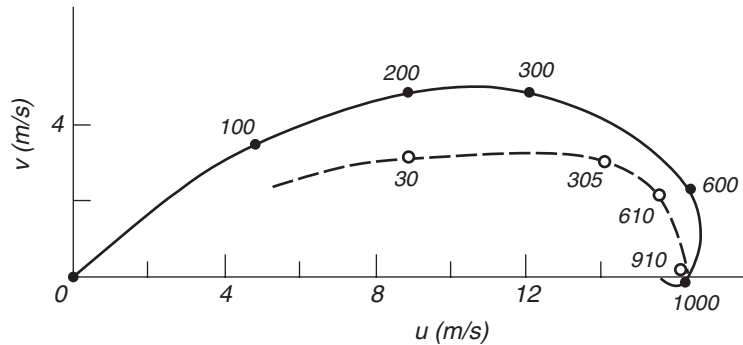
Figure 9.4 Ekman layer for the lowest kilometer in the atmosphere (solid line), together with wind velocity measured by Dobson (1914) - - -. The numbers give height above the surface in meters. The boundary layer at the bottom of the ocean has a similar shape. (From Houghton, 1977).
