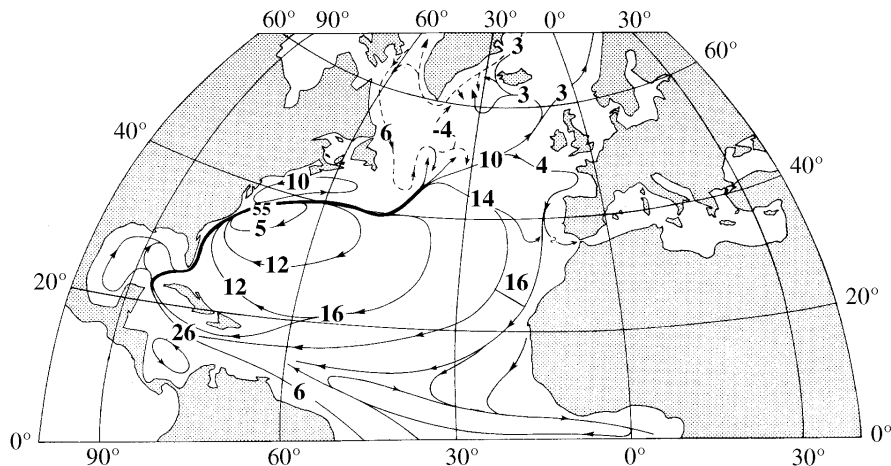
Figure 11.8 Sketch of the major surface currents in the North Atlantic. Values are transport in units of 10^6 \text{ m}^3/\text{s} (From Sverdrup, Johnson, and Fleming 1942: fig. 187).
