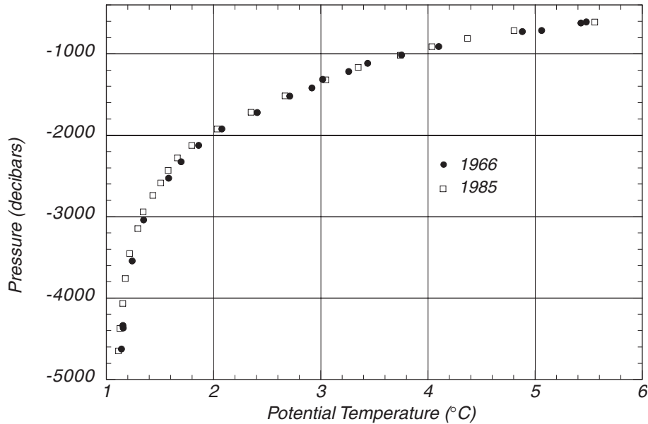
Figure 8.8 Potential temperature measured as a function of depth (pressure) near 24.7^{\circ}\text{N} , 161.4^{\circ}\text{W} in the central North Pacific by the Yaquina in 1966 (●), and by the Thompson in 1985 (□). Data from Atlas of Ocean Sections produced by Swift, Rhines, and Schlitzer.
