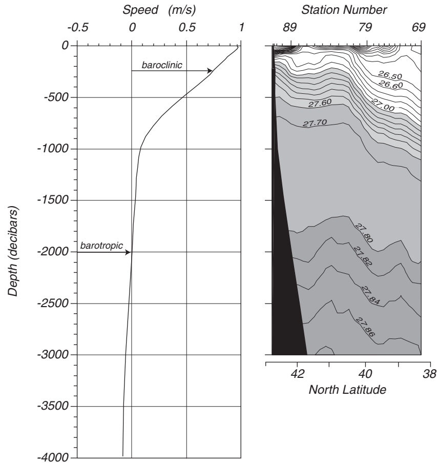
Figure 10.8 Left Relative current as a function of depth calculated from hydrographic data collected by the Endeavor cruise south of Cape Cod in August 1982. The Gulf Stream is the fast current shallower than 1000 decibars. The assumed depth of no motion is at 2000 decibars. Right Cross section of potential density \sigma_\theta across the Gulf Stream along 63.66^\circ\text{W} calculated from CTD data collected from Endeavor on 25–28 April 1986. The Gulf Stream is centered on the steeply sloping contours shallower than 1000m between 40^\circ and 41^\circ . Notice that the vertical scale is 425 times the horizontal scale. (Data contoured by Lynn Talley, Scripps Institution of Oceanography).
