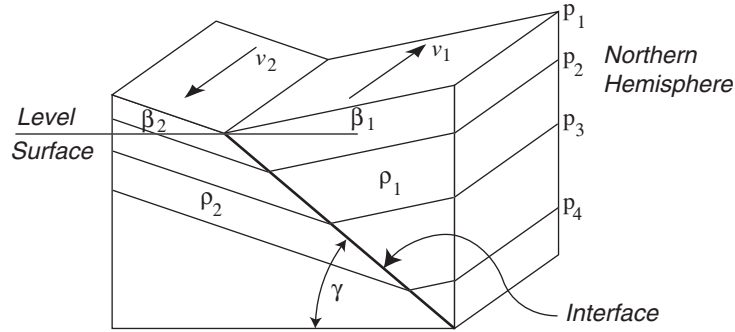
Figure 10.11 Slopes \beta of the sea surface and the slope \gamma of the interface between two homogeneous, moving layers, with density \rho_1 and \rho_2 in the northern hemisphere.
