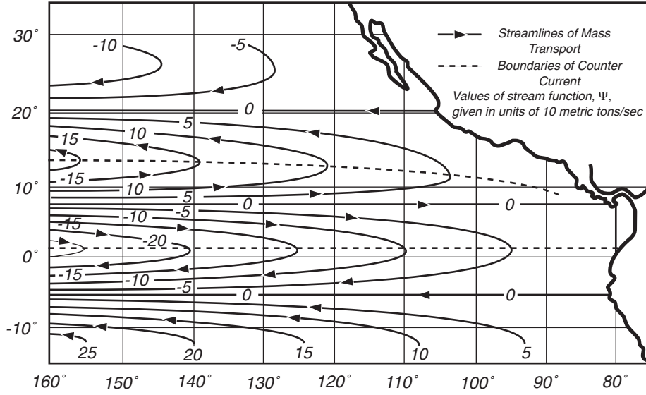
Figure 11.1 Streamlines of mass transport in the eastern Pacific calculated from Sverdrup's theory using mean annual wind stress (From Reid 1948).
