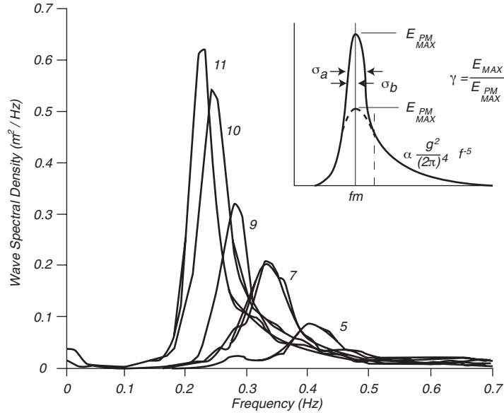
Figure 16.9 Wave spectra of a developing sea for different fetches according to Hasselmann et al. (1973).
