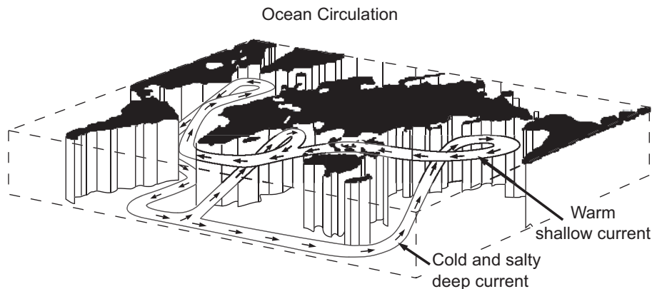
Figure 13.1 The oceanic conveyor belt carries heat northward into the north Atlantic. Note that this is a cartoon, and it does not accurately describe the ocean's circulation. (from Broecker and Peng, 1982).
