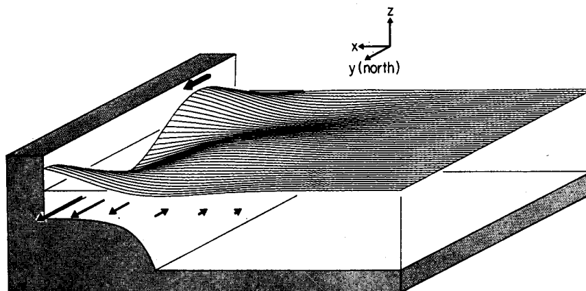
Figure 17.6 Computer-assisted sketch of an edge wave. Such waves exist in the breaker zone near the beach and on the continental shelf. (From Cutchin and Smith, 1973).
