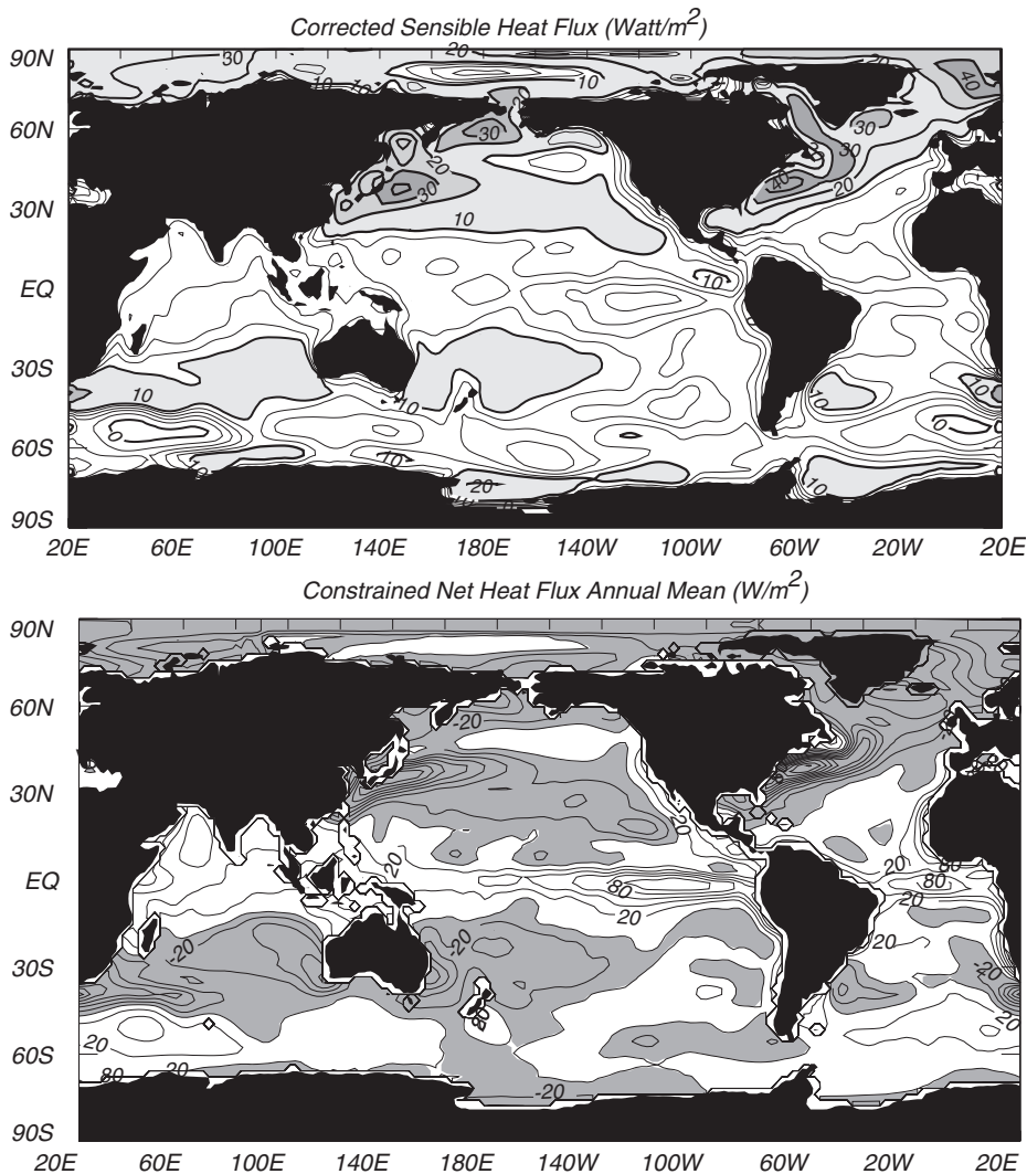
Figure 5.10 Annual-mean upward sensible heat flux Q_S Top and constrained, net, downward heat flux Bottom through the sea surface in W/m^2 calculated by DaSilva, Young, and Levitus (1995) using the COADS data set from 1945 to 1989. Contour interval is 2 W/m^2 (top) and 20 W/m^2 (bottom).
