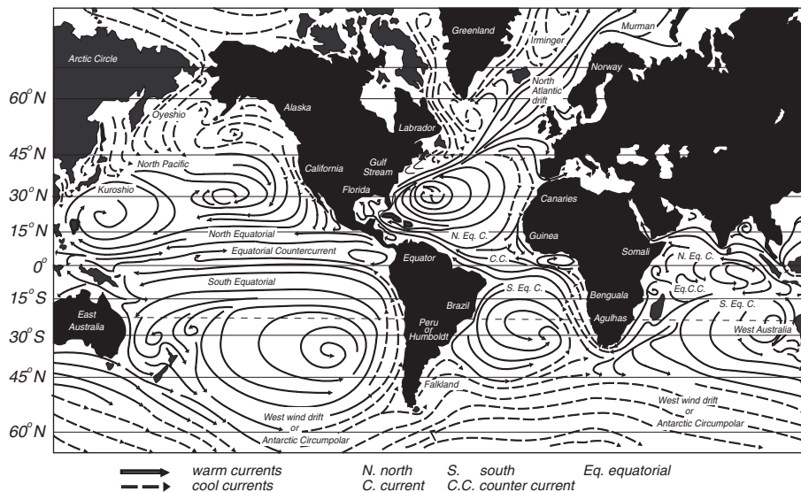
Figure 2.8 The time-averaged, surface circulation of the ocean deduced from nearly a century of oceanographic expeditions (From Tolmazin, 1985).
