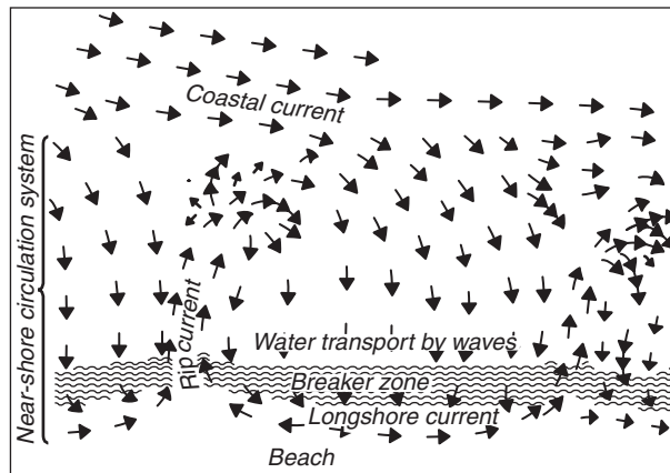
Figure 17.5 Sketch of rip currents generated by water carried to the beach by breaking waves (From Dietrich, Kalle, Krauss, & Siedler, 1980).
