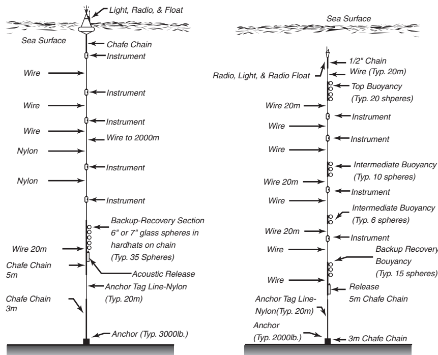
Figure 10.18 Left: An example of a surface mooring of the type deployed by the Woods Hole Oceanographic Institution's Buoy Group. Right: An example of a subsurface mooring deployed by the same group. (From Baker, 1981).
