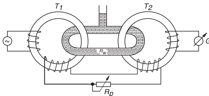
Figure 6.13 The induction method measurement of electrical conductivity uses a sea-water loop which couples two transformer loops T_1 and T_2 . The induced voltage in the second loop is proportional to conductivity R_w of the water. From Dietrich et al. 1980.
