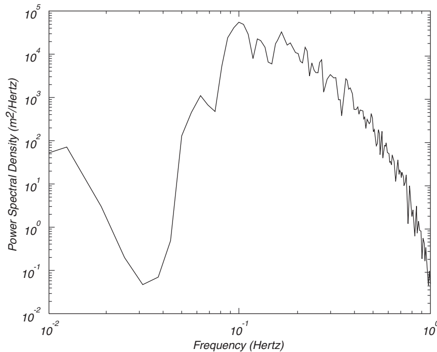
Figure 16.6 The spectrum of waves calculated from 11 minutes of data shown in figure 7.2 by averaging four periodograms to reduce uncertainty in the spectral values. Spectral values below 0.04 Hz are in error due to noise.
