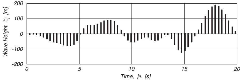
Figure 16.3 The first 20 seconds of digitized data from figure 16.2. \Delta = 0.32 s.
