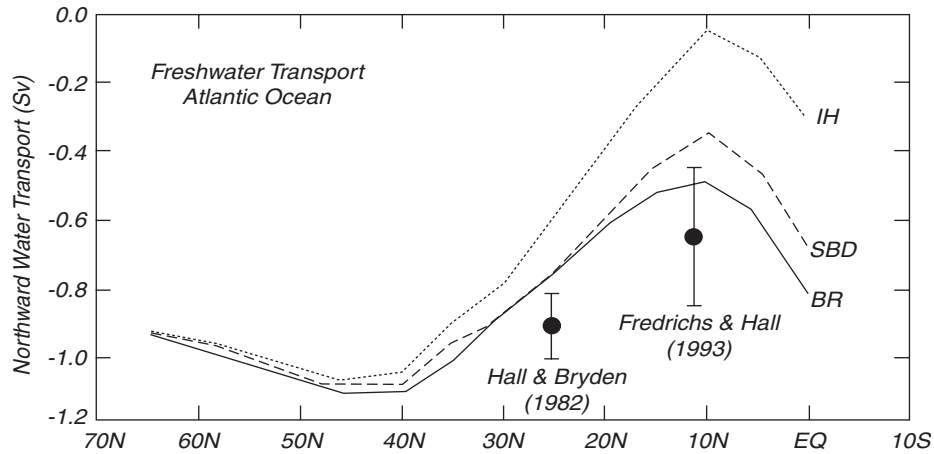
Figure 5.13 Meridional transport of fresh water by the Atlantic from three surface-flux calculations: BR—Baumgartner and Reichel (1975); SBD—Schmitt et al. (1989); and IH—Isemer and Hasse's (1987) evaporation estimates combined with Dorman and Bourke's (1981) precipitation values. Also shown are direct measurements at 24°N by Hall and Bryden (1982) and 11°N by Friedrichs and Hall (1993). All are summed relative to an estimated Arctic southward export due to the Bering Strait through flow and the water budget of the Arctic itself. From Schmitt (1994).
