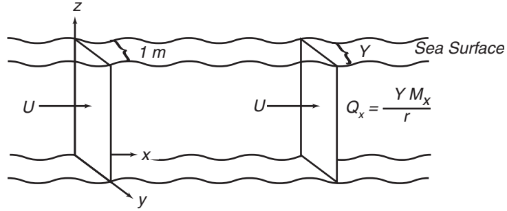
Figure 9.7 Sketch for defining Left: mass transports, and Right: volume transports.
