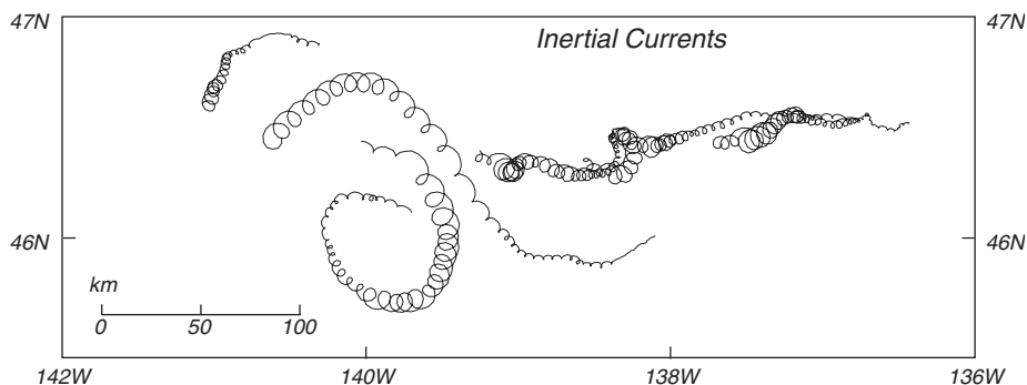
Figure 9.1 Inertial currents in the North Pacific in October 1987 (days 275–300) measured by holey-sock drifting buoys drogued at a depth of 15 meters. Positions were observed 10–12 times per day by the Argos system on NOAA polar-orbiting weather satellites and interpolated to positions every three hours. The largest currents were generated by a storm on day 277. Note these are not individual eddies. The entire surface is rotating. A drogue placed anywhere in the region would have the same circular motion. From van Meurs (1998).
