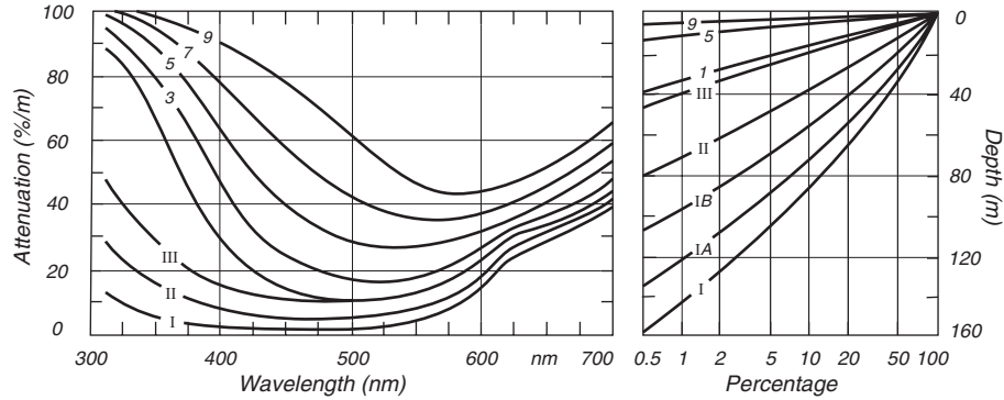
Figure 6.18 Left: Attenuation of daylight in the ocean in % per meter as a function of wavelength. I: extremely pure ocean water; II: turbid tropical-subtropical water; III: mid-latitude water; 1-9: coastal waters of increasing turbidity. Incidence angle is 90^\circ for the first three cases, 45^\circ for the other cases. (From Jerlov, 1951). Right: Percentage of 465 nm light reaching indicated depths for the same types of water. (From Jerlov, 1968).
