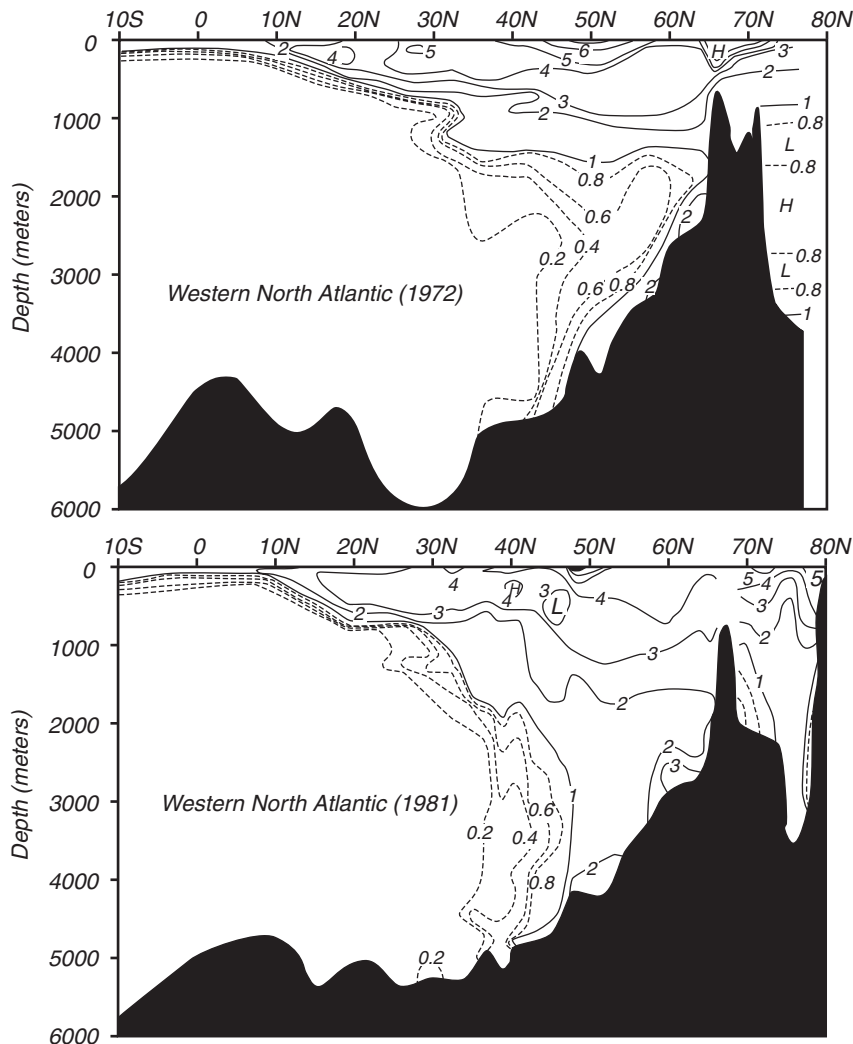
Figure 10.15 Distribution of tritium along a section through the western basins in the North Atlantic, measured in 1972 ( Top ) and remeasured in 1981 ( Bottom ). Units are tritium units, where one tritium unit is 10^{18} (tritium atoms)/(hydrogen atoms) corrected to the activity levels that would have been observed on 1 January 1981. Compare this figure to the density in the ocean shown in figure 13.9. From Toggweiler (1994)
