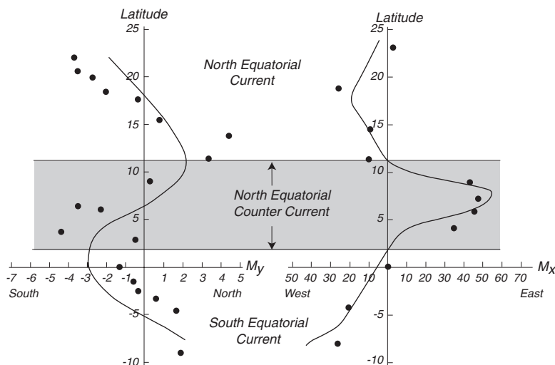
Figure 11.2 Mass transport in the eastern Pacific calculated from Sverdrup's theory using observed winds with 11.9 and 11.11 (solid lines) and pressure calculated from hydrographic data from ships with 11.4 (dots). Transport is in tons per second through a section one meter wide extending from the sea surface to a depth of one kilometer. Note the difference in scale between M_y and M_x (From Reid, 1948).
