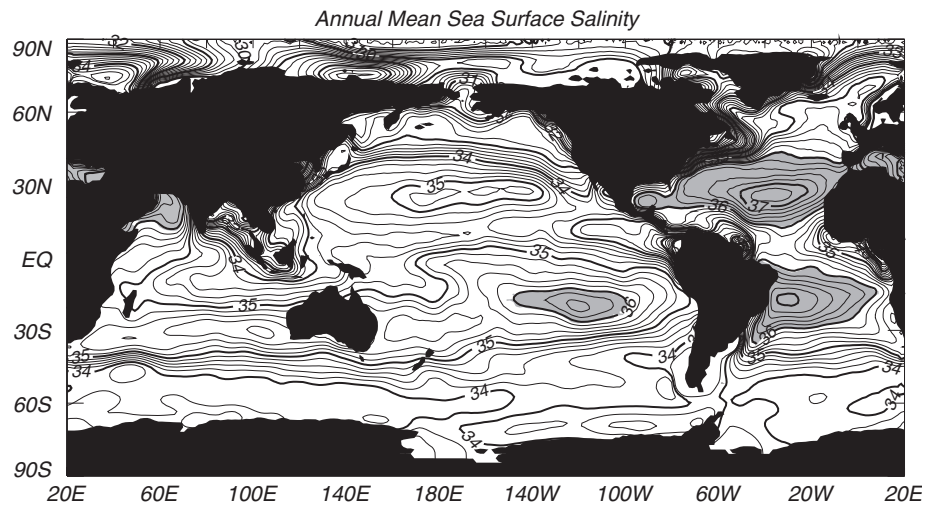
Figure 6.4 Mean sea-surface salinity. Contour interval is 0.25 psu. Shaded areas exceed 36 psu. (From Levitus, 1982).
