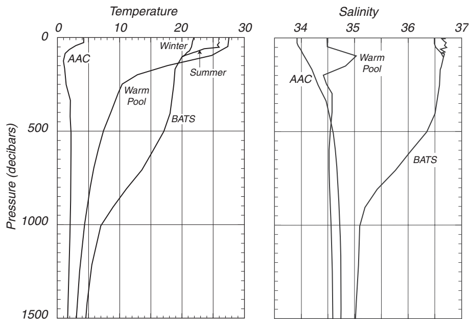
Figure 6.8 Typical temperature and salinity profiles in the open ocean. AAC: At 62.0^{\circ} S, 170.0^{\circ} E in the Antarctic Circumpolar Current on 16 January 1969 as measured by the R/V Hakuho Maru . Warm Pool: At 9.5^{\circ} N 176.3^{\circ} E in the tropical west Pacific warm pool on 12 March 1989 as measured by Bryden and Hall on the R/V Moana Wave . BATS: At 31.8^{\circ} N 64.1^{\circ} W near Bermuda on 17 April and 10 September 1990 as measured by the Bermuda Biological Station for Research, Inc. Data are included with Java OceanAtlas.
