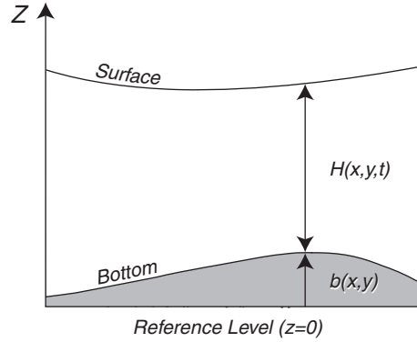
Figure 12.1 Sketch of fluid flow used for deriving conservation of potential vorticity (From Cushman-Roisin, 1994).
