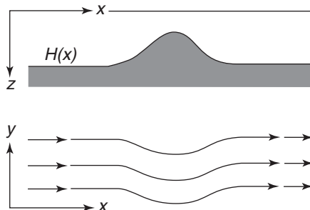
Figure 12.4 Barotropic flow over a sub-sea ridge is turned equatorward to conserve potential vorticity (from Dietrich, et al. , 1980).
