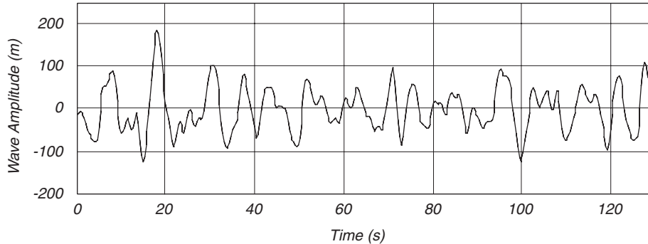
Figure 16.2 A short record of wave amplitude measured by a wave buoy in the North Atlantic.
