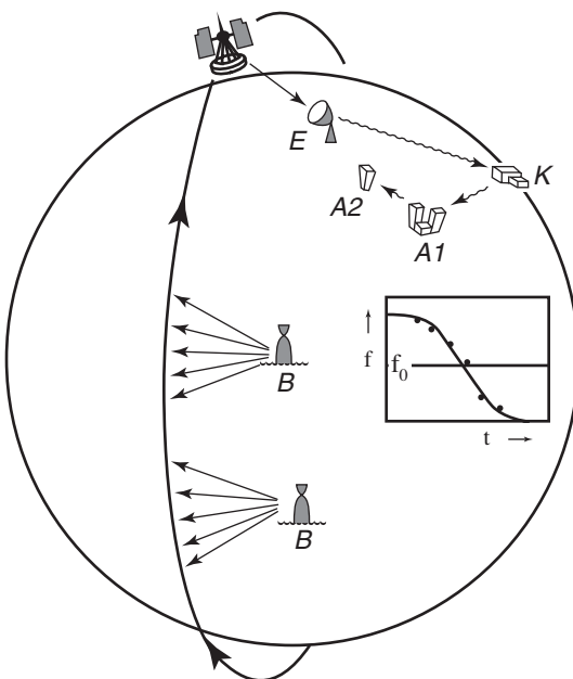
Figure 10.13 Satellite systems, especially System Argos, use radio signals transmitted from surface buoys to determine the position of the buoy. The satellite S receives a radio signal from the buoy B . The time rate of change of the signal, the Doppler shift, is a function of buoy position and distance from the satellite's track. The recorded Doppler signal is transmitted to ground stations E , which relays the information to processing centers A via control stations K . (From Dietrich et al. , 1980)
