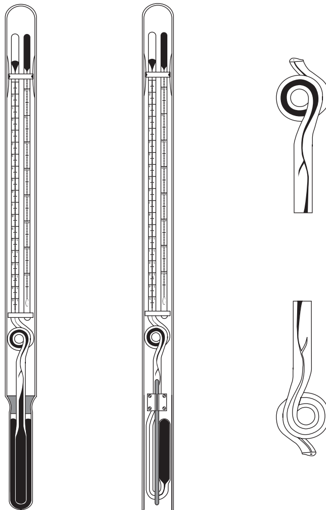
Figure 6.11 Left: Protected and unprotected reversing thermometers in set position, before reversal. Right: The constricted part of the capillary in set and reversed positions (From von Arx, 1962).
