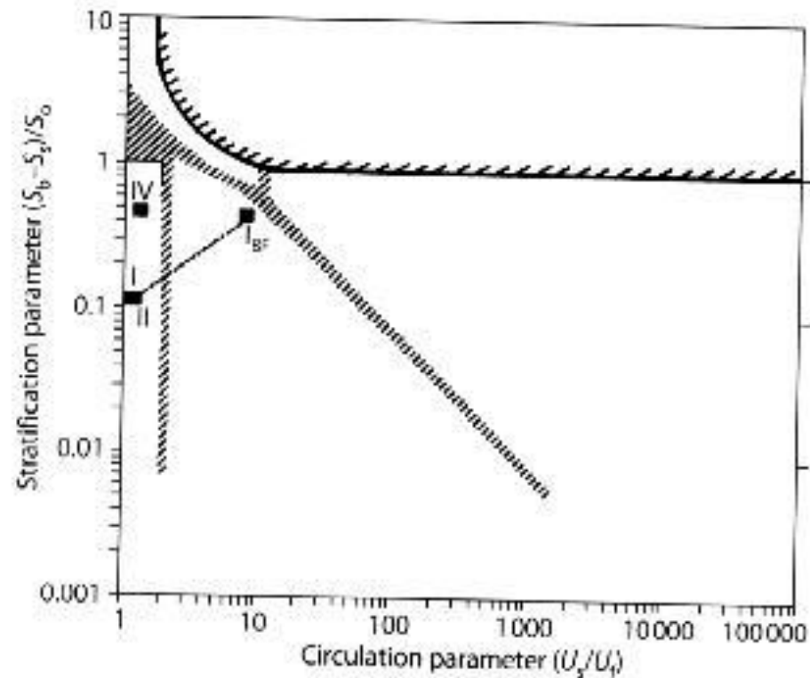
Fig. 5.10. The stratification/circulation diagram for the situations of PLATES I, II and IV. The index "BF" refers to PLATES I data obtained before the meteorological front passage
