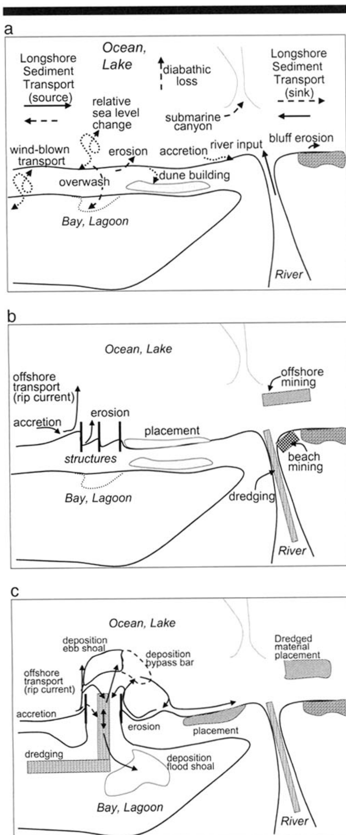
Figure 3. Possible sediment transport pathways for different types of coastal regions (a) Natural beach, (b) Engineered beach, (c) Inlet and adjacent beaches (Note: All pathways illustrated for the natural beach (a) also apply to the engineered beach (b), and all those shown for both the natural and engineered beaches apply to the inlet case (c)).
