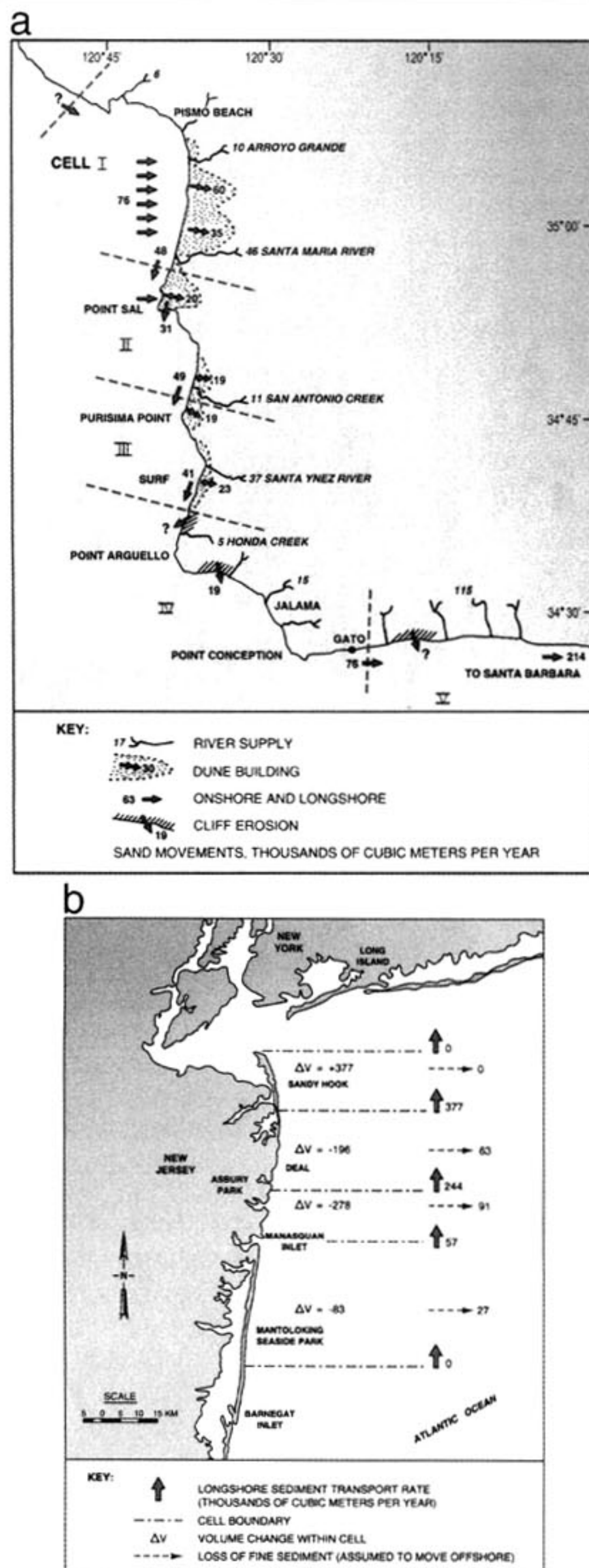
Figure 1. Early sediment budgets (a) Southern California sediment budget (adapted from Bowen and Inman 1966), (b) North New Jersey sediment budget (adapted from Caldwell 1966).
