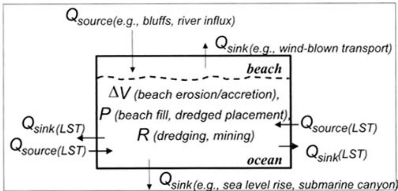
Figure 2. Sediment budget parameters as may enter Equation (1).
