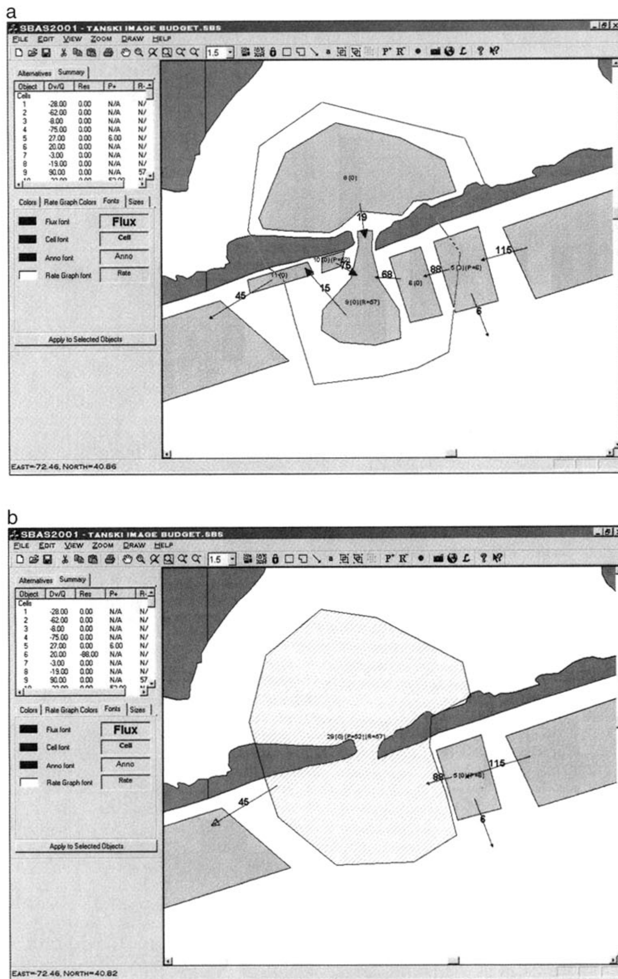
Figure 8. Collapsing cells within SBAS. (a) Polygonal selection for collapsing cells, (b) collapsed sediment budget cells for Shinnecock Inlet.
